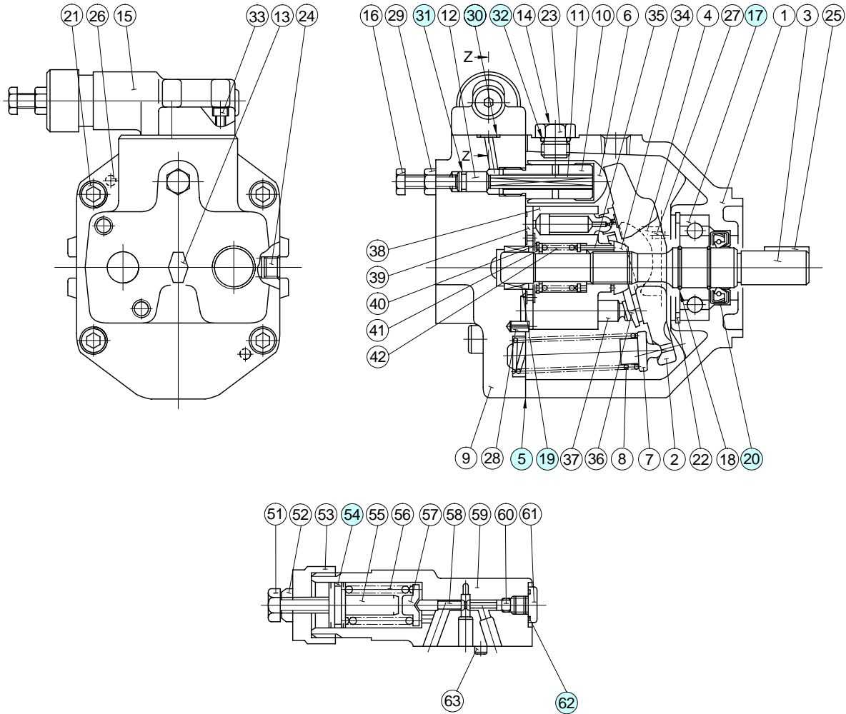
Section Z-Z
